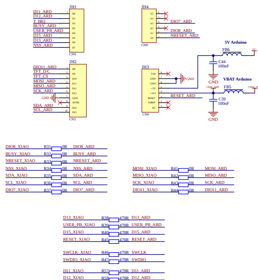
Arduino-LR2021 Headers
